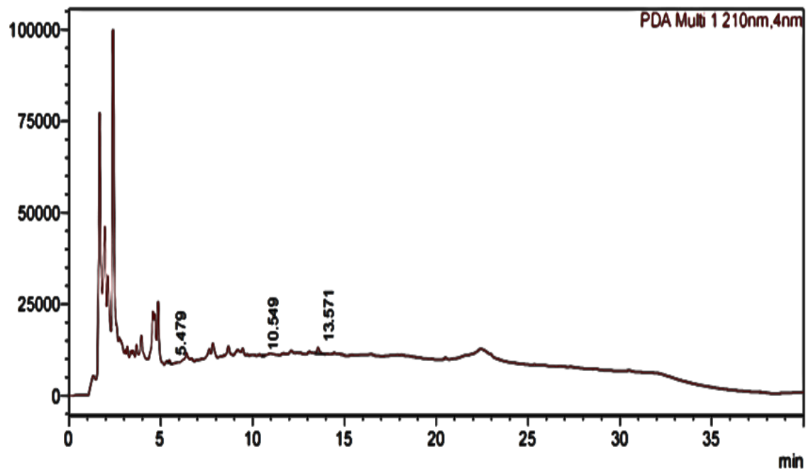
Graph 5: HPLC analysis of Udupi
