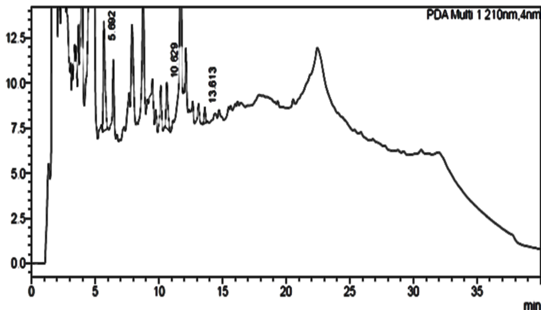
Graph 9: HPLC analysis of Bagalkote
