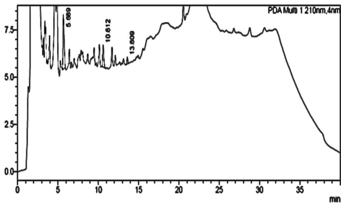
Graph 8: HPLC analysis of Ballari
