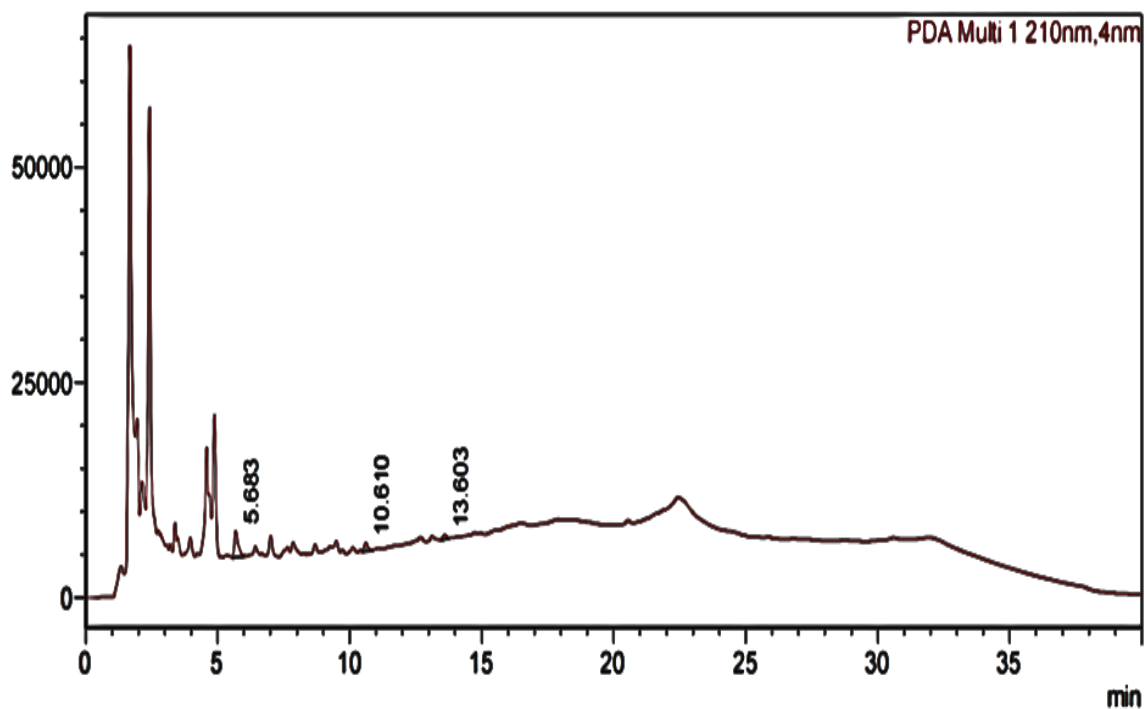
Graph 3: HPLC analysis of Shivamogga
