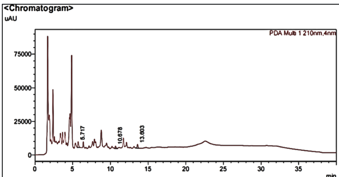
Graph 2: HPLC analysis of Chitradurga
