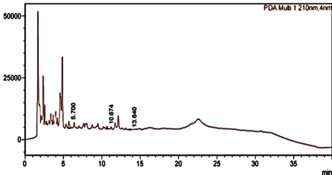
Graph 1: HPLC analysis of Davanagere
