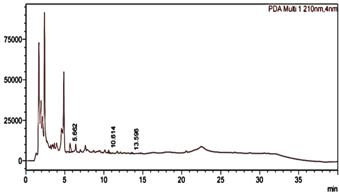
Graph 4: HPLC analysis of Mysuru
