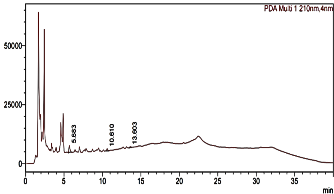
Graph 7: HPLC analysis of Belagavi
