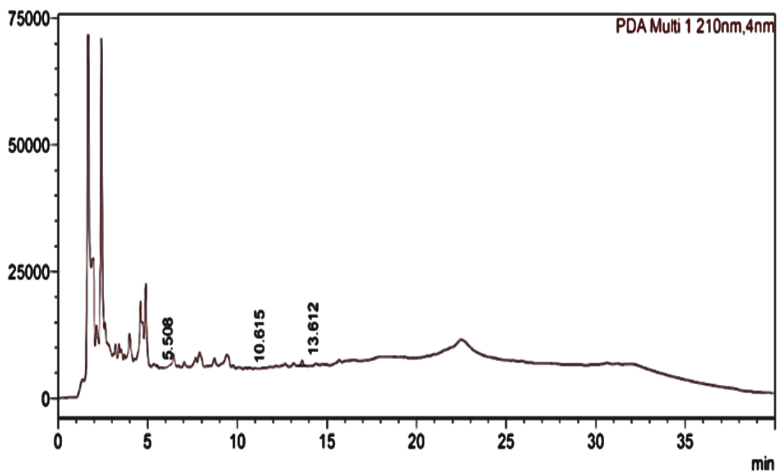
Graph 6: HPLC analysis of Chikkamagaluru
