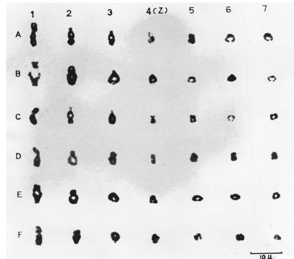
Figure 8: Partial karyotype of diplotene / diakinesis of T. p. phoenicoptera A and B – standard karyotype 1 m 1 m /2 st 2 st ); C and D – heterozygous karyotype (1 m 1 m /2 st 2 st ); E and F - inversion homozygous karyotype (1 m 1 m /2 m 2 m )
